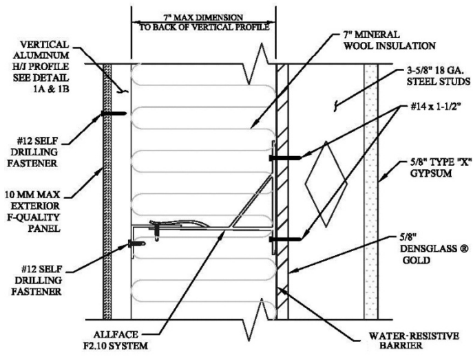
④ MAXIMUM INSULATION CAVITY DEPTH
